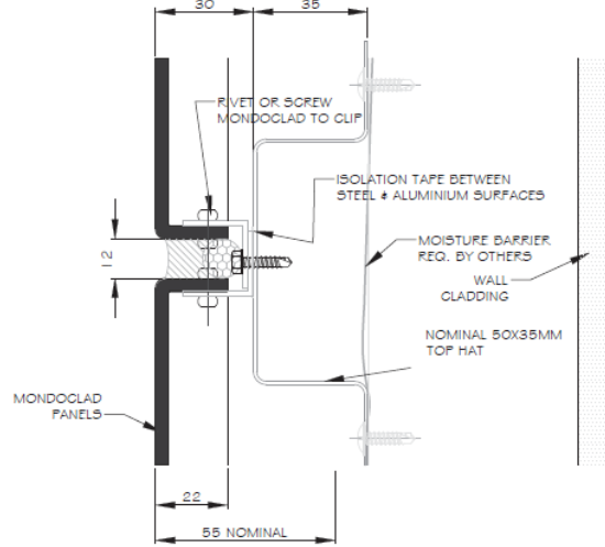
04 HORIZONTAL JOINT DETAIL
