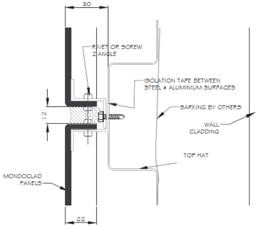
04 HORIZONTAL JOINT DETAIL Z ANGLE
