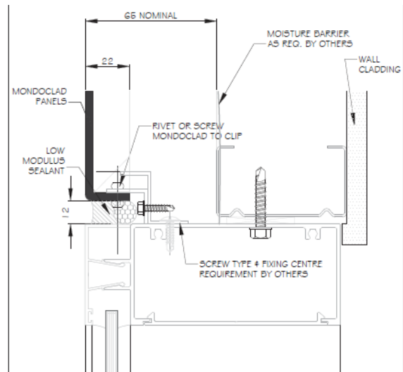
02 WINDOW HEAD DETAIL
