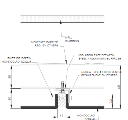
05 VERTICAL JOINT
